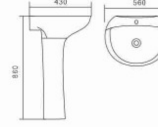
P21 22" Basin With Pedestal Size: 560×430×860mm Fixing with back to wall Vitreous china
