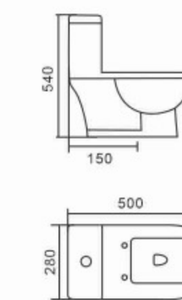
823 Washdown Separated Toilet Size: 500 x 280x 540mm S-trap,150mm Roughing-in
