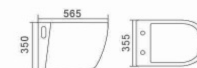
887 Washdown Wall hung closet Size:565x355x350mm Vitreous china
