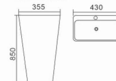
A206 Basin With Pedestal Size: 430x355x850mm Fixing with back to wall Vitreous china
