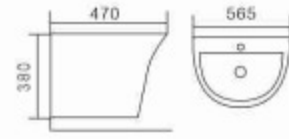
P45 Wall-hang Basin Size: 565×470×380mm Wall-hung Installation
