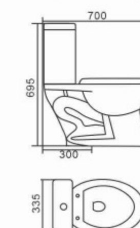
8994 Siphonic Separated Toilet Bowl & Tank Size: 700x335x695mm S-trap, 300mm Roughing-in
