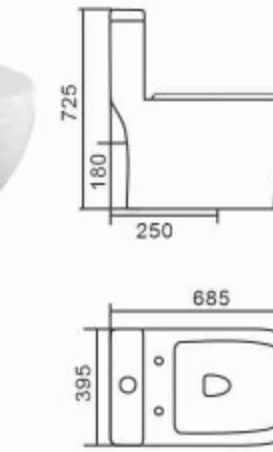
438 Washdown One-piece Toilet Size: 685 x 395x 725mm S-trap,250mm Roughing-in P-trap,180mm Roughing-in
