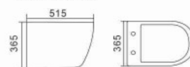
880 Wall hung Toilet Flushing system:Rimless Size:515x365x365mm Vitreous china
