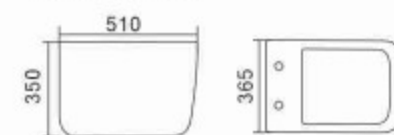
889 Wall hung Toilet Flushing system:Rimless Size:510x365x350mm Vitreous china
