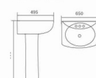
P28 Basin With Pedestal Size: 650×495×850mm Fixing with back to wall Vitreous china
