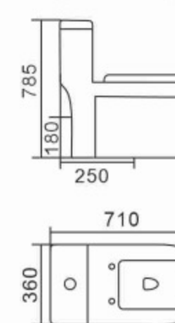
362W Washdown One-piece Toilet Size: 710 x 360 x 785mm S-trap,250mm Roughing-in P-trap,180mm Roughing-in
