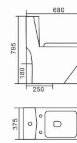
363 Washdown One-piece Toilet Size: 680 x 375x 795mm S-trap,250mm Roughing-in P-trap,180mm Roughing-in
