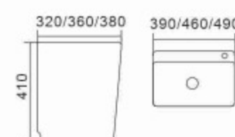
D37 Mop Tub Size:390×320×410mm 460×360×410mm 490×380×410mm Vitreous china Fixing with back to wall
