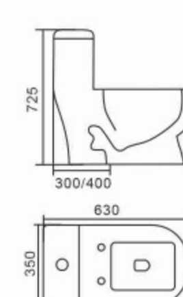
392 Siphonic One-piece Toilet Size: 630 x 350x 725mm S-trap,300/400mm Roughing-in
