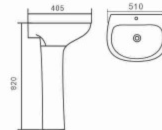
P20 Basin With Pedestal Size: 510×405×820mm Fixing with back to wall Vitreous china
