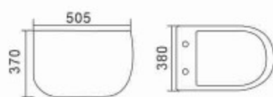
881 Wall hung Toilet Flushing system:Rimless Size:505x380x370mm Vitreous china
