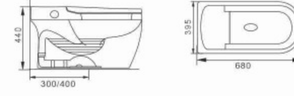
844 Smart Toilet Siphonic Bowl & Tank Size: 680 x395x440mm S-trap,300/400mm Roughing-in
