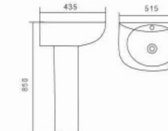
P56 21" Basin With Pedestal Size: 515×435×850mm Fixing with back to wall Vitreous china
