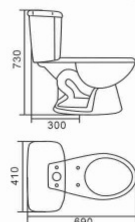
861 Siphonic Separated Toilet Bowl & Tank Size: 690x410x730mm S-trap, 300mm Roughing-in
