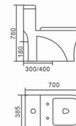
402 Siphonic One-piece Toilet Size: 700 x 385x 780mm S-trap,300/400mm Roughing-in P-trap,180mm Roughing-in
