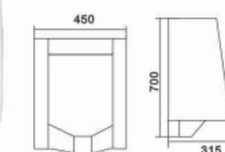
D05 Wall-hung Urinal Size:450×315×700mm Wall Mounted outlet or floor Mounted outlet spud Installation
