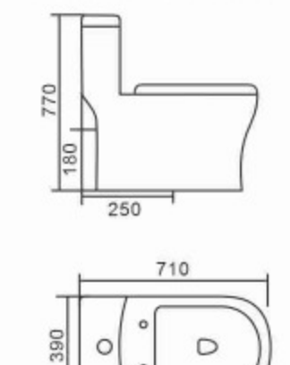
422 Washdown One-piece Toilet Size: 710 x 390x 770mm S-trap,250mm Roughing-in P-trap,180mm Roughing-in
