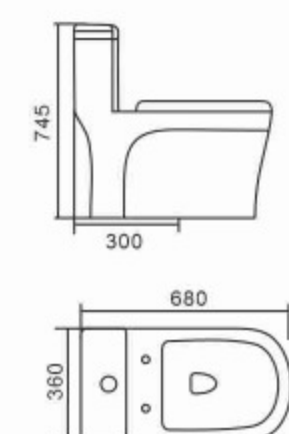
385 Siphonic One-piece Toilet Size: 680 x 360 x 745mm S-trap,300mm Roughing-in
