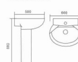
P32 Basin With Pedestal Size: 660×500×880mm Fixing with back to wall Vitreous china
