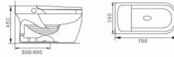
840 Smart Toilet Siphonic Bowl & Tank Size: 700 x390x450mm S-trap,300/400mm Roughing-in
