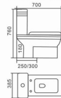
345 Washdown One-piece Toilet Size: 700 x 385 x 760mm S-trap,250/300mm Roughing-in P-trap,180mm Roughing-in
