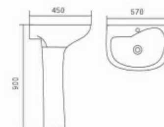
P04 22" Basin With Pedestal Size: 570×450×900mm Fixing with back to wall Vitreous china
