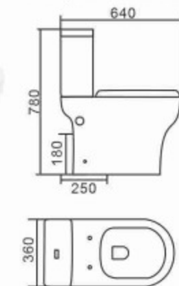
897 Washdown Separated Toilet Bowl & Tank Size: 640x360x780mm S-trap, 250mm Roughing-in P-trap, 180mm Roughing-in
