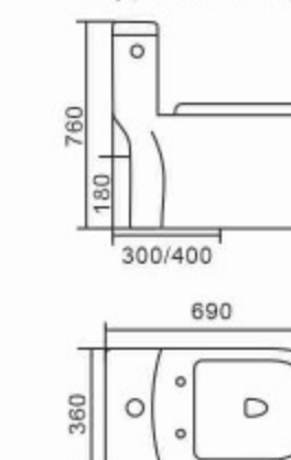
405 Siphonic One-piece Toilet Size: 690 x 360x 760mm S-trap,300/400mm Roughing-in P-trap,180mm Roughing-in
