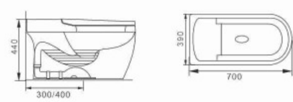
845 Smart Toilet Siphonic Bowl & Tank Size: 700 x390x440mm S-trap,300/400mm Roughing-in
