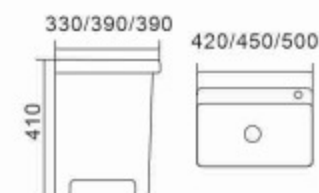
D36 Do laundry the plank Size:420×330×410mm 450×390×410mm 500×390×410mm Vitreous china Fixing with back to wall
