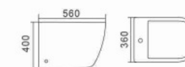
DB883 Bidet Size:560x360x400mm Vitreous china
