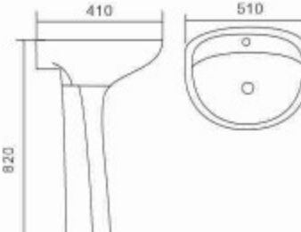
P03 20" Basin With Pedestal Size: 510×410×820mm Fixing with back to wall Vitreous china
