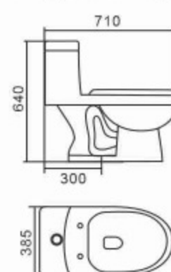
316B Siphonic One-piece Toilet Size: 710 x 385 x 640mm S-trap,300mm Roughing-in
