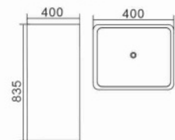
A204A Basin With Pedestal Size: 400x400x835mm Fixing with back to wall Vitreous china
