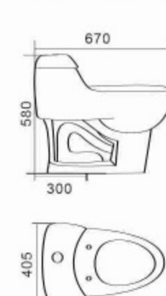
328 Siphonic One-piece Toilet Size: 670 x 405 x 580mm S-trap,300mm Roughing-in
