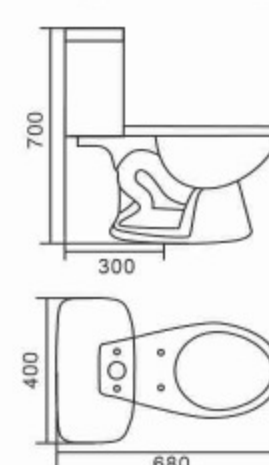
895 Siphonic Separated Toilet Bowl & Tank Size: 680x400x700mm S-trap, 300mm Roughing-in
