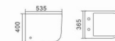
B888 Washdown Floor standing Toilet Size:535x365x400mm Vitreous china
