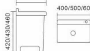
D38 Mop Tub Size:400×330×420mm 500×360×430mm 600×400×460mm Vitreous china Fixing with back to wall
