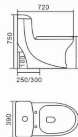
347 Washdown One-piece Toilet Size: 720 x 390 x 750mm S-trap,250/300mm Roughing-in P-trap,180mm Roughing-in
