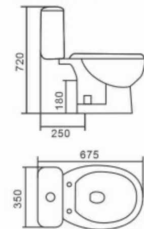
841 Washdown Separated Toilet Bowl & Tank Size: 675x350x720mm S-trap, 250mm Roughing-in P-trap, P-trap45°
