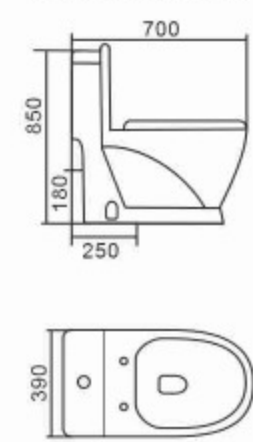
355 Washdown One-piece Toilet Size: 700 x 390 x 850mm S-trap,250mm Roughing-in P-trap,180mm Roughing-in
