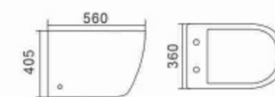
B883 Washdown Floor standing Toilet Size:560x360x405mm Vitreous china
