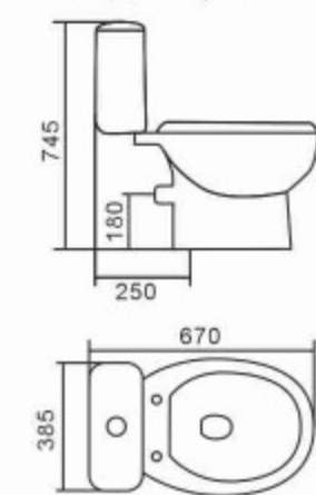
858 Washdown Separated Toilet Bowl & Tank Size: 670x385x745mm S-trap, 250mm Roughing-in P-trap, P-trap45°
