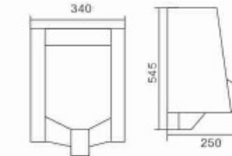
D02 Wall-hung Urinal Size:340×250×545mm Wall Mounted outlet or floor Mounted outlet spud Installation
