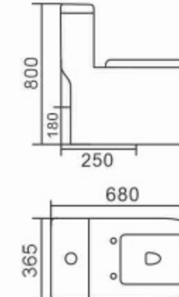
358 Washdown One-piece Toilet Size: 680 x 365 x 800mm S-trap,250mm Roughing-in P-trap,180mm Roughing-in
