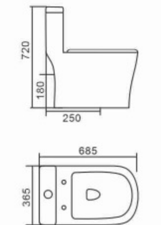
439 Washdown One-piece Toilet Size: 685 x 365x 720mm S-trap,250mm Roughing-in P-trap,180mm Roughing-in
