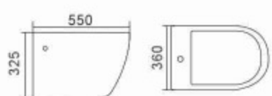
D882 Bidet Size:550x360x325mm Vitreous china
