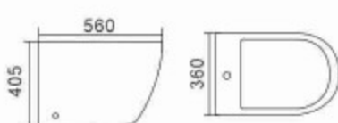
DB882 Bidet Size:560x360x405mm Vitreous china
