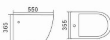
A882 Washdown Wall hung closet Size:550x355x365mm Vitreous china
