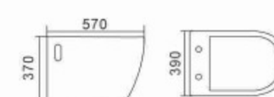
884 Wall hung Toilet Flushing system:Rimless Size:570x390x370mm Vitreous china
