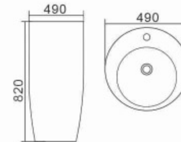
A203 Basin With Pedestal Size: 490x490x820mm Fixing with back to wall Vitreous china
