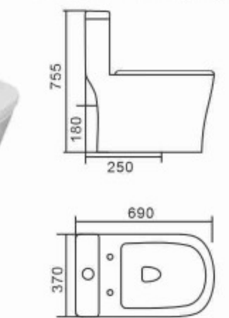
442 Washdown One-piece Toilet Size: 690 x 370x 755mm S-trap,250mm Roughing-in P-trap,180mm Roughing-in
