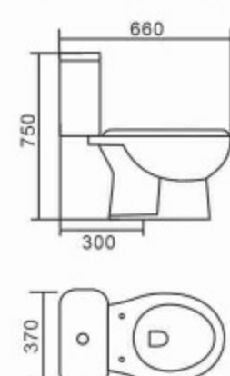
852 Siphonic Separated Toilet Bowl & Tank Size: 660x370x750mm S-trap, 300mm Roughing-in
