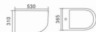
D888 Bidet Size:530x365x310mm Vitreous china
