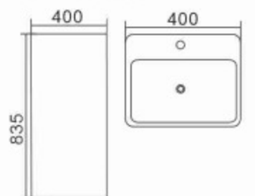
A204 Basin With Pedestal Size: 400x400x835mm Fixing with back to wall Vitreous china
