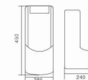
D62 Wall-hung Urinal Size:285×240×490mm Wall Mounted outlet or floor Mounted outlet spud Installation
