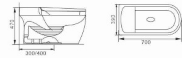
841 Smart Toilet Siphonic Bowl & Tank Size: 700 x390x470mm S-trap,300/400mm Roughing-in
