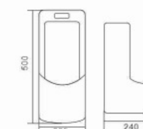
D62B Wall-hung Urinal Size:285×240×500mm Wall Mounted outlet or floor Mounted outlet spud Installation
