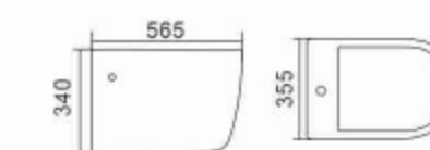
D883 Wall hung Bidet Size:565x355x340mm Vitreous china
