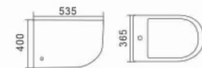
DB888 Bidet Size:535x365x400mm Vitreous china
