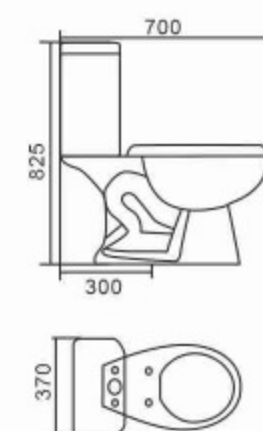
851 Siphonic Separated Toilet Bowl & Tank Size: 700x370x825mm S-trap, 300mm Roughing-in
