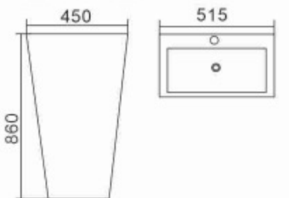
A205 Basin With Pedestal Size: 515x450x860mm Fixing with back to wall Vitreous china
