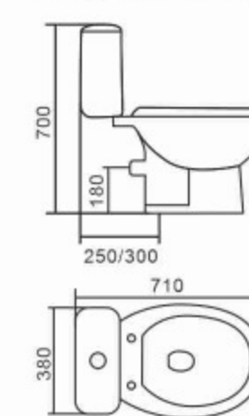
839 Washdown Separated Toilet Bowl & Tank Size: 710x380x700mm S-trap, 250/300mm Roughing-in P-trap, 180mm Roughing-in
