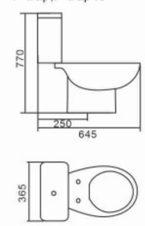
8315 Washdown Separated Toilet Bow & Tank Size: 645x365x770mm S-trap, 250mm Roughing-in P-trap, P-trap45°
