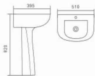
P19 Basin With Pedestal Size: 510×395×820mm Fixing with back to wall Vitreous china
