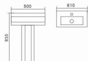
P05 Basin With Pedestal Size: 610×500×835mm Fixing with back to wall Vitreous china
