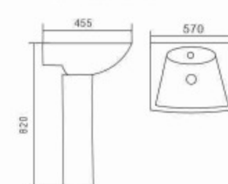
P27 Basin With Pedestal Size: 570×455×820mm Fixing with back to wall Vitreous china
