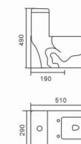
821 Siphonic One-piece Toilet Size: 510 x 290x490mm S-trap,190mm Roughing-in
