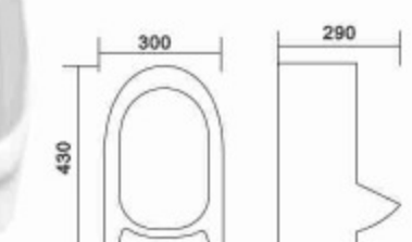
D10 Wall-hung Urinal Size:300×290×430mm Wall Mounted outlet or floor Mounted outlet spud Installation
