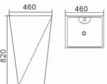
A207 Basin With Pedestal Size: 460x460x820mm Fixing with back to wall Vitreous china
