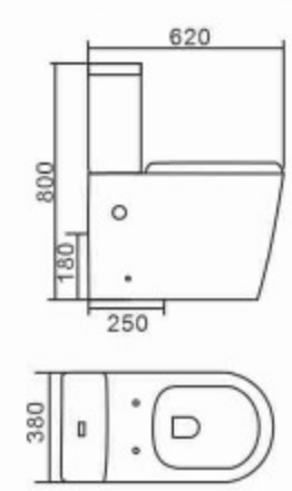
902 Washdown Separated Toilet Bowl & Tank Size: 620x380x800mm S-trap, 250mm Roughing-in P-trap, 180mm Roughing-in
