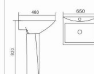
P34 Basin With Pedestal Size: 650×480×820mm Fixing with back to wall Vitreous china
