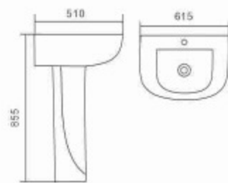
P09 Basin With Pedestal Size: 615×510×855mm Fixing with back to wall Vitreous china
