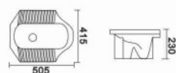
D35 Squaffing Pan Size:505×415×230mm Installation into the earth
