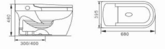
839 Smart Toilet Siphonic Bowl & Tank Size: 680 x395x480mm S-trap,300/400mm Roughing-in
