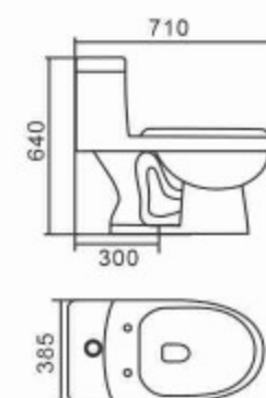
316 Siphonic One-piece Toilet Size: 710 x 385 x 640mm S-trap,300mm Roughing-in
