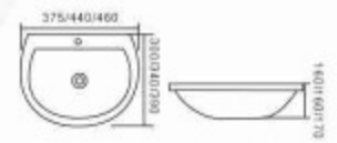
P03 14"16"18" Hang-Basin Size: 375×300×160mm 440×340×160mm 460×390×170mm
