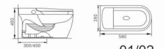
830 Smart Toilet Siphonic Bowl & Tank Size:580 x380x450mm S-trap,300/400mm Roughing-in
