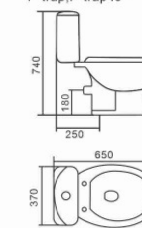
8312 Washdown Separated Toilet Bowl & Tank Size: 650x370x740mm S-trap, 250mm Roughing-in P-trap, P-trap45°
