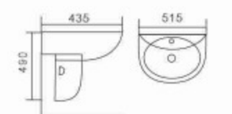
P56W Half pedestal basin Size: 515×435×490mm Wall-hung Installation
