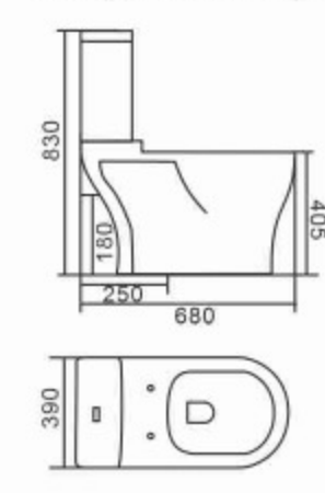
890 Washdown Separated Toilet Bowl & Tank Size: 680x390x830mm S-trap, 250mm Roughing-in P-trap, 180mm Roughing-in
