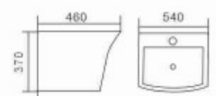
P43 Wall-hang Basin Size: 540×460×370mm Wall-hung Installation
