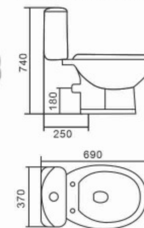
833 Washdown Separated Toilet Bowl & Tank Size: 690x370x740mm S-trap, 250mm Roughing-in P-trap, 180mm Roughing-in
