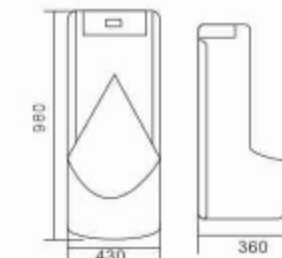
D23 Wall-hung Urinal Size:430×360×980mm Wall Mounted outlet or floor Mounted outlet spud Installation
