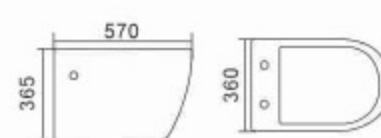
A883 Washdown Wall hung closet Size:570x360x365mm Vitreous china
