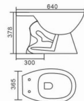
857 Siphonic Toilet Bowl & Tank Size: 640x365x378mm S-trap, 300mm Roughing-in Vitreous china
