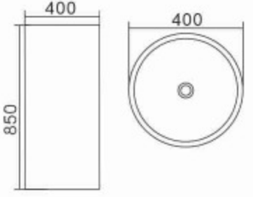
A202A Basin With Pedestal Size: 400x400x850mm Fixing with back to wall Vitreous china
