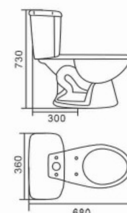
860 Siphonic Separated Toilet Bowl & Tank Size: 680x360x730mm S-trap, 300mm Roughing-in
