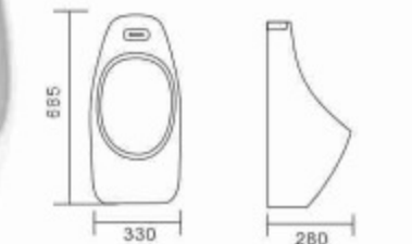
D47 Wall-hung Urinal Size:330×280×685mm Wall Mounted outlet or floor Mounted outlet spud Installation
