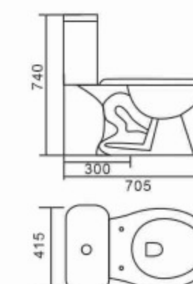
898 Siphonic Separated Toilet Bowl & Tank Size: 705x415x740mm S-trap, 300mm Roughing-in
