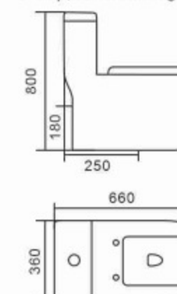
359 Washdown One-piece Toilet Size: 660 x 360 x 800mm S-trap,250mm Roughing-in P-trap,180mm Roughing-in
