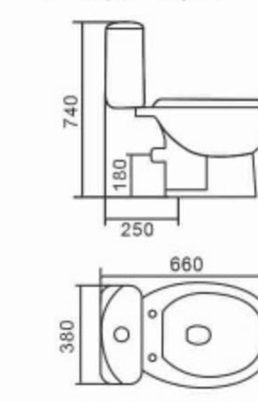
8318 Washdown Separated Toilet Bowl & Tank Size: 660x380x740mm S-trap, 250mm Roughing-in P-trap, P-trap45°
