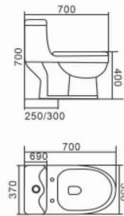
012 Washdown One-piece Toilet Size: 700 x 370 x 700mm S-trap,250/300mm Roughing-in
