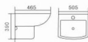
P44 Wall-hang Basin Size: 505×465×390mm Wall-hung Installation
