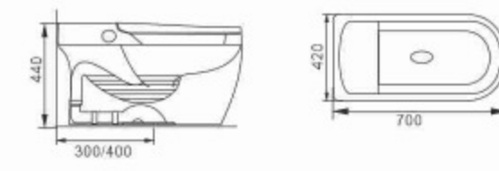
831 Smart Toilet Siphonic Bowl & Tank Size:700 x420x440mm S-trap,300/400mm Roughing-in
