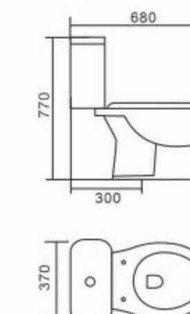
8902 Siphonic Separated Toilet Bowl & Tank Size: 680x370x770mm S-trap, 300mm Roughing-in
