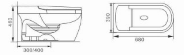
842 Smart Toilet Siphonic Bowl & Tank Size: 680 x390x460mm S-trap,300/400mm Roughing-in
